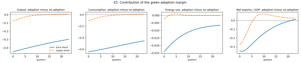
Figure 3: Contribution of the green adoption margin (full minus frozen), by shock. Output, consumption, energy use, net exports.
