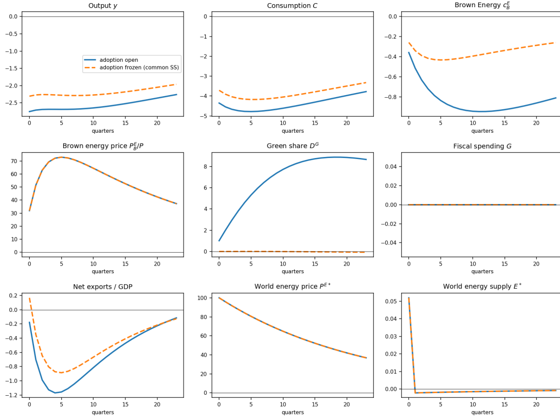
E1a. Brown energy PRICE shock (ARS-style, elastic supply)
