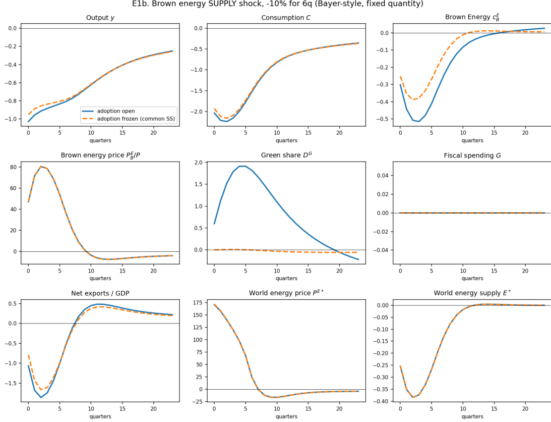
Figure 2: Brown energy supply shock ( -10\% for 6 quarters, fixed quantity), adoption open (solid) vs. frozen (dashed), no policy.
