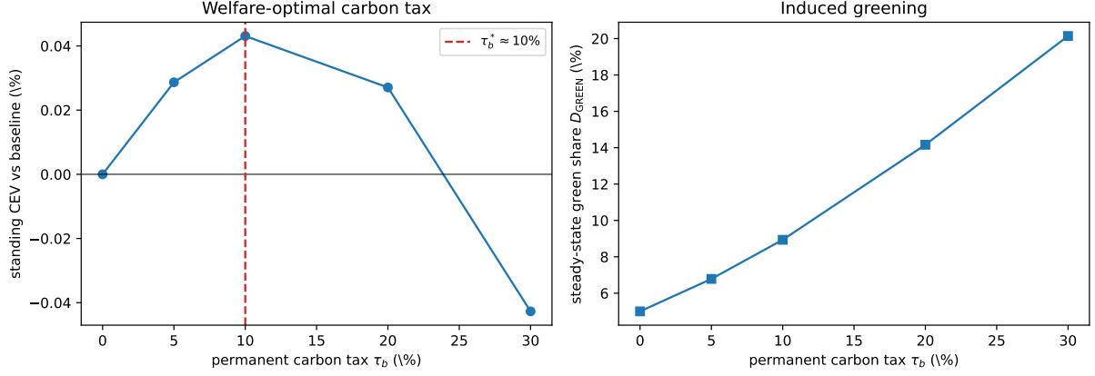
Figure 7: The welfare-optimal permanent carbon tax. Left: standing CEV of the \tau_b steady state relative to the no-tax baseline (no crisis), hump-shaped with an interior optimum near \tau_b^* \approx 10\% . Right: the induced steady-state green share D_{ss}^G . \psi_g is held fixed; the carbon revenue is rebated lump-sum.
