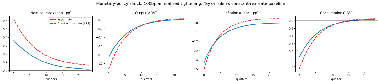
Figure 14: Monetary-policy shock (100bp annualised tightening): Taylor rule (solid) versus the constant-real-rate baseline (dashed). Nominal rate, output, inflation, consumption.
