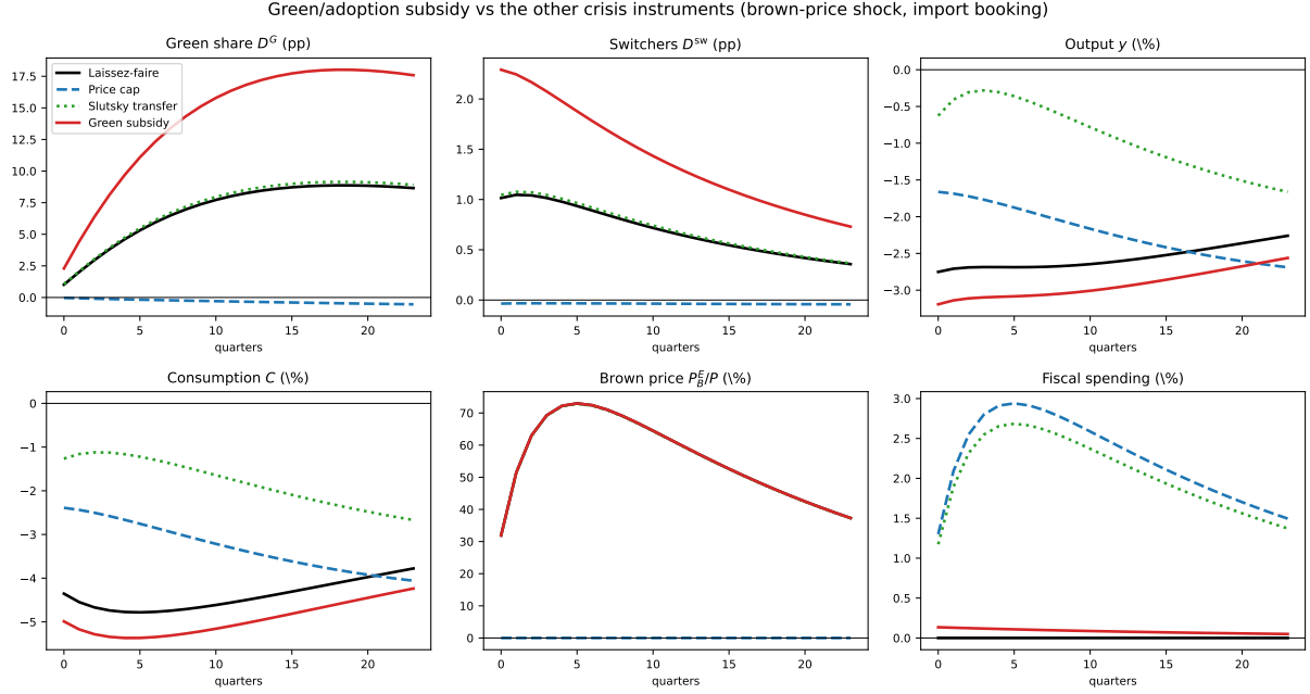
Figure 8: The green/adoption subsidy at the trough, against laissez-faire, the price cap and the Slutsky transfer (brown-price shock). It doubles the adoption response ( D^G , D^{sw} ) at trivial fiscal cost, yet forcing the real switching cost in the middle of the consumption crisis leaves output and private welfare below laissez-faire.
